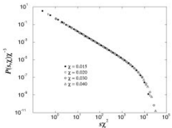
FIG. 3. The distribution of avalanche sizes in the infinite range model as a function of \chi for N = 32696 and \bar{c} = 0 . The data collapse is obtained from the scaling function P(s, \chi) = s^{-3/2}f(\chi^2 s) .
